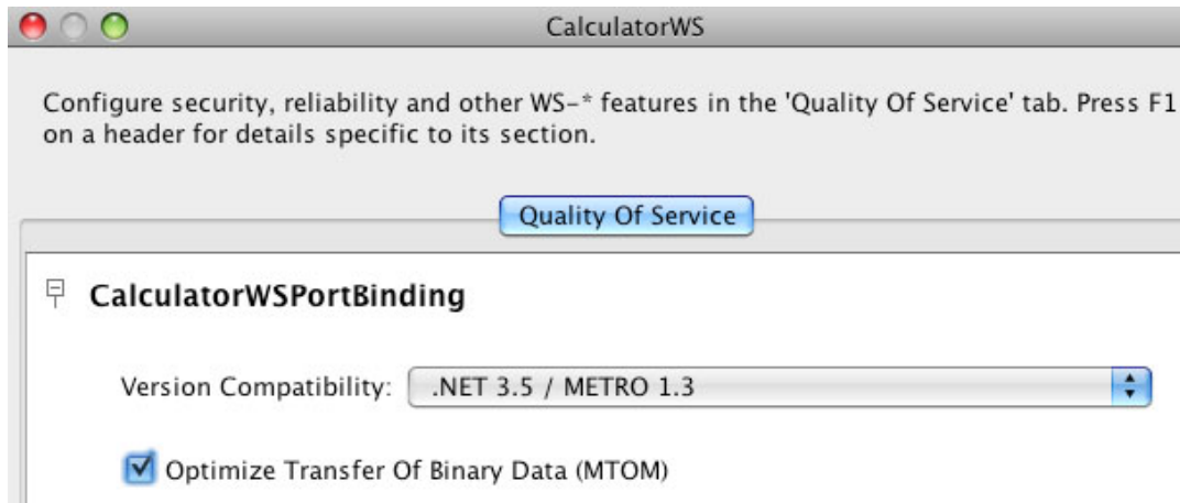
Figure 8.1. Enabling MTOM
